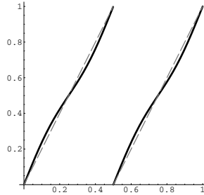
FIGURE 4. Non-Bernoulli example and the one-sided \{\frac{1}{2}, \frac{1}{2}\} Bernoulli (dotted line).
