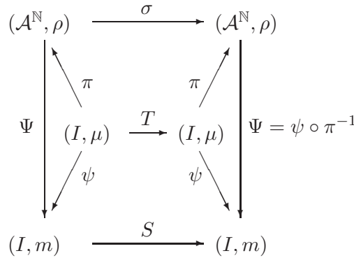
FIGURE 2. Commutative diagram to construct \Psi = \psi \circ \pi^{-1} .
